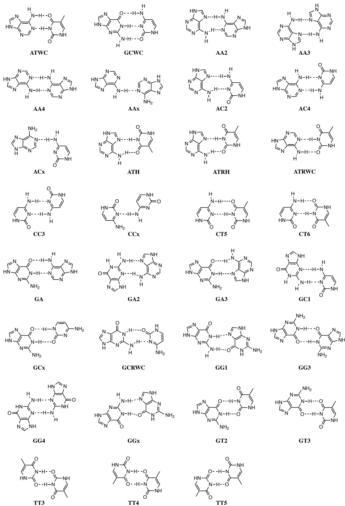
Scheme 1. Watson Crick and mismatched base pairs.
