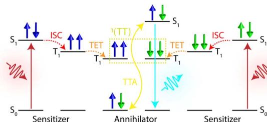
Fig. 1 The TTA-UC cascade that begins by the sensitizers absorbing low energy photons and undergoing intersystem crossing (ISC) to yield excited triplet states. Triplet energy transfer (TET) then occurs between the sensitizer and annihilator. When two triplet excited annihilators come into contact, triplet–triplet annihilation (TTA) may occur, which, through an intermediate triplet pair state, can yield a ground state and an annihilator in its singlet excited state that ultimately emits the upconverted photon.
