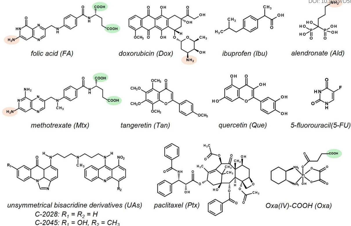
Fig. 2 Structures of folic acid and drugs tested in QD-based hybrid drug nanocarriers.
