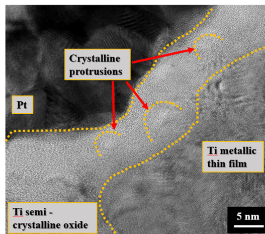
Fig. 8 TEM image of the anodic memristor grown on a Ti thin film with the Pt top electrode (adapted from ref. 24).
