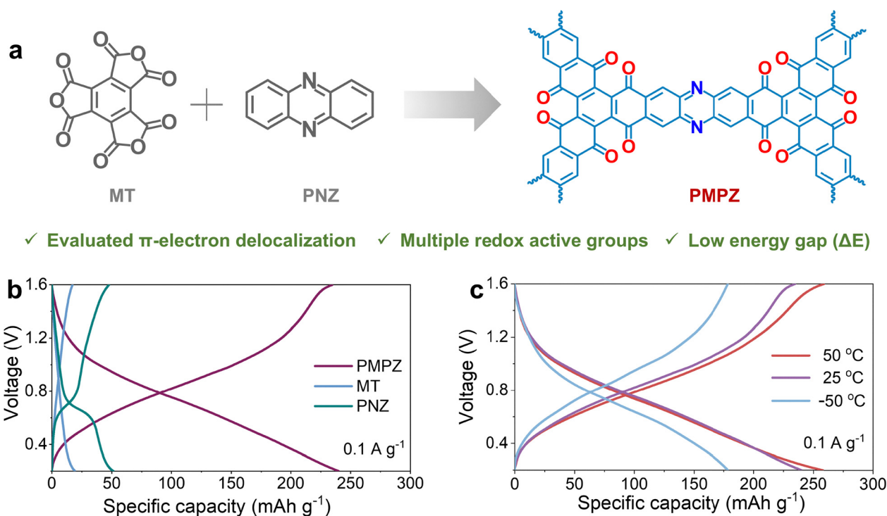
Fig. 1 (a) Synthesis diagram of PMPZ. (b) Charge/discharge curves of MT, PNZ, and PMPZ at 0.1 \text{ A g}^{-1} . (c) Charge/discharge curves of PMPZ at 0.1 \text{ A g}^{-1} at 50 °C, 25 °C, and -50 °C.
