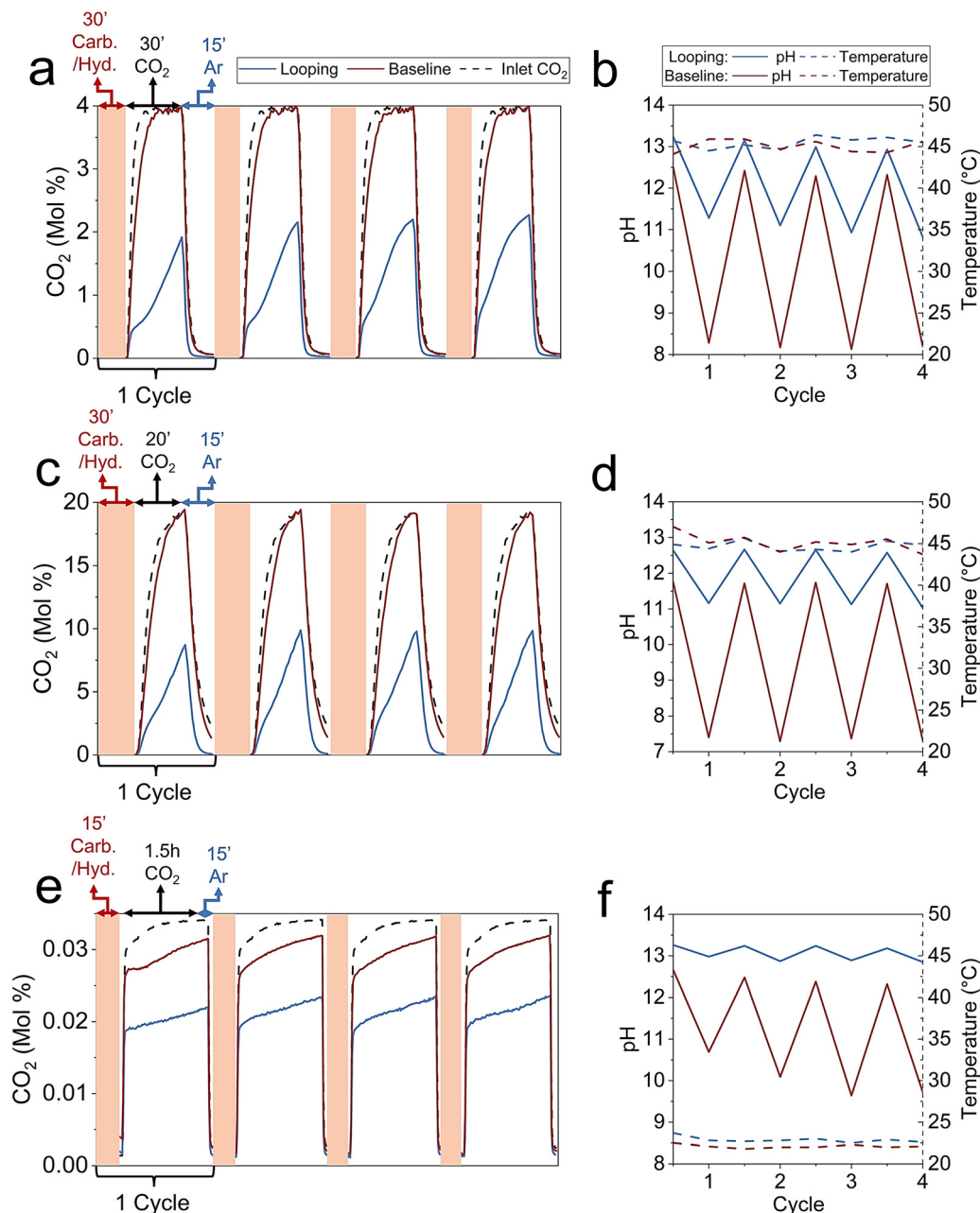
Fig. 2 (a) Four \text{Na}_2\text{CO}_3 looping cycles of 4% \text{CO}_2 with quenched BOF slag compared to the baseline; the conditions were 1 g slag per cycle, 45^{\circ}\text{C} , and 90 sccm 4% \text{CO}_2/\text{Ar} . (b) pH and temperature after each step in 4% \text{CO}_2 looping and baseline. Half cycles are after carbonation and full cycles are after \text{CO}_2 capture. (c) Four \text{Na}_2\text{CO}_3 looping cycles of 20% \text{CO}_2 with aged fines BOF slag compared to the baseline; the conditions were 10 g slag per cycle, 45^{\circ}\text{C} , and 90 sccm 20% \text{CO}_2/\text{Ar} . (d) pH and temperature after each step in 20% \text{CO}_2 looping and baseline. (e) Four \text{Na}_2\text{CO}_3 looping cycles of air \text{CO}_2 with quenched BOF slag compared to the baseline; the conditions were 0.05 g slag per cycle, 24^{\circ}\text{C} , and 90 sccm 343 ppm \text{CO}_2 . (f) pH and temperature after each step in air \text{CO}_2 looping and baseline.
