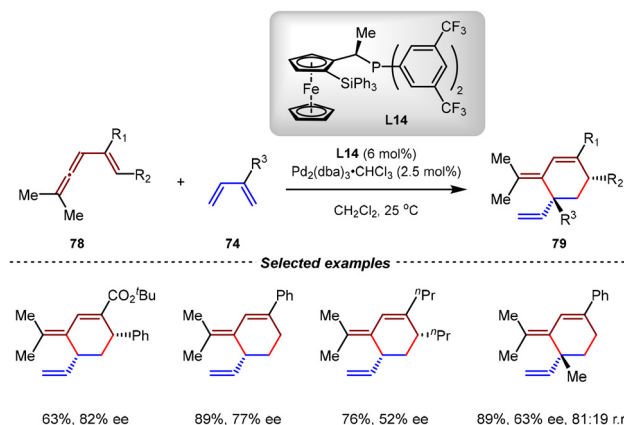
Scheme 21 \text{Pd}(0) -catalyzed asymmetric intermolecular [4+2] cycloadditions of vinylallenes and 1,3-dienes.
