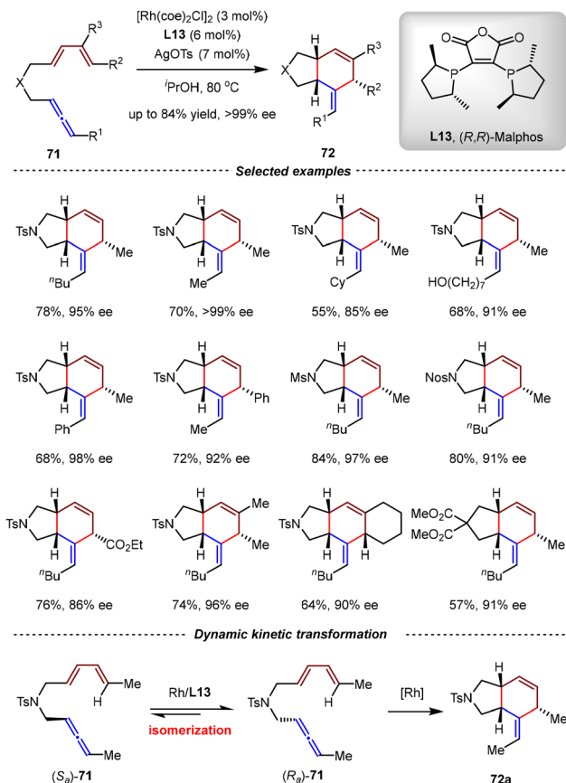
Scheme 19 Rh(I)/Malphos-catalyzed dynamic kinetic resolution (DKR) of racemic allene-1,3-dienes via the intramolecular [4+2] cycloaddition.
