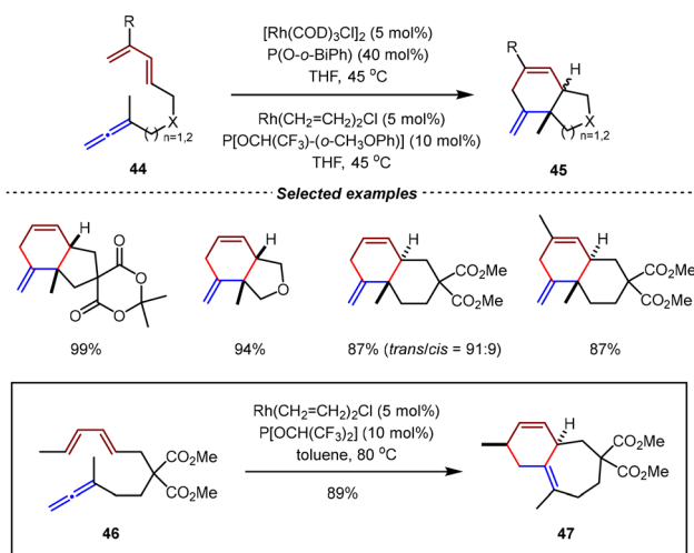
Scheme 14 Rh(I)/phosphite-catalyzed intramolecular [4+2] cycloaddition of 1,1-disubstituted allene-1,3-dienes.
