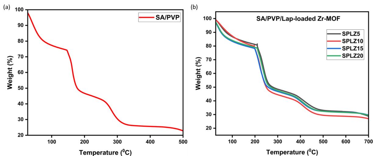
Fig. 11 TGA of: (a) optimized SA/PVP film (90 : 10) and (b) different weight percentages of SA/PVP/Lap-loaded Zr-MOF (5%, 10%, 15%, and 20% of lapatinib-loaded Zr-MOF with the optimized SA/PVP blend (90 : 10 SA/PVP), labelled as SPLZ5, SPLZ10, SPLZ15, and SPLZ20, respectively).
