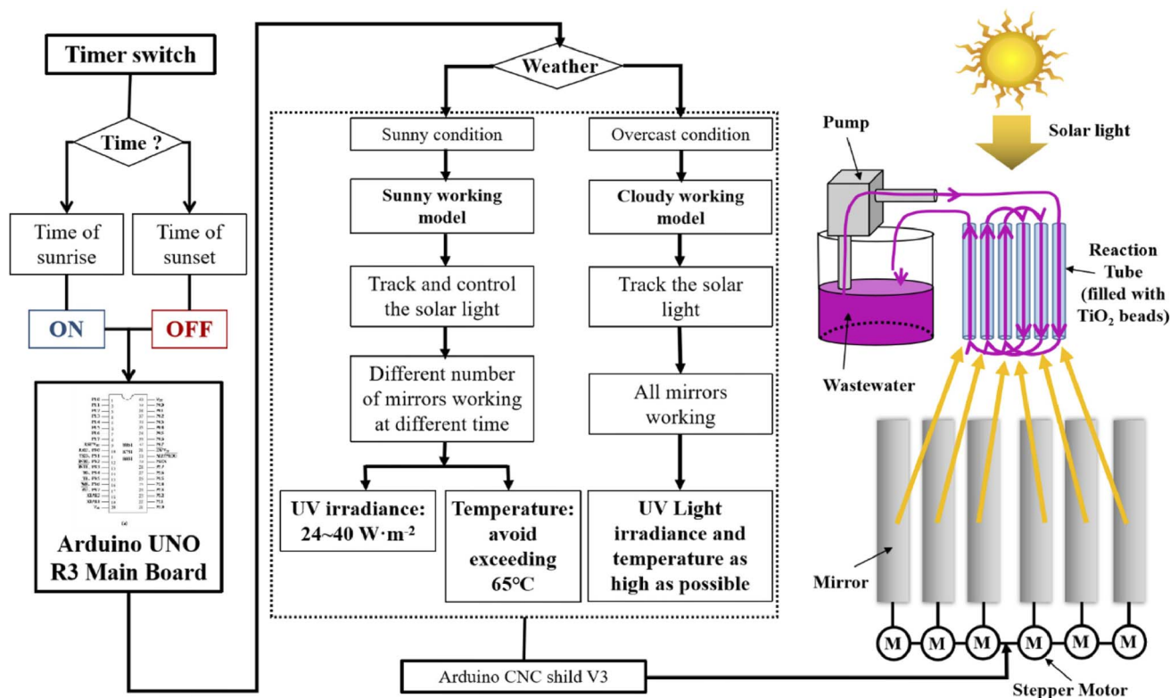
Fig. 11 The flow chart of the LFP control system. Reproduced from ref. 240 with permission from MDPI.
