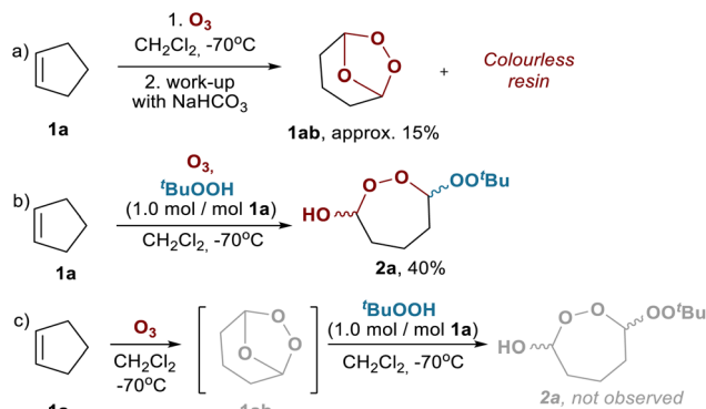
Scheme 3 Initial experiments on cyclopentene ozonolysis.
