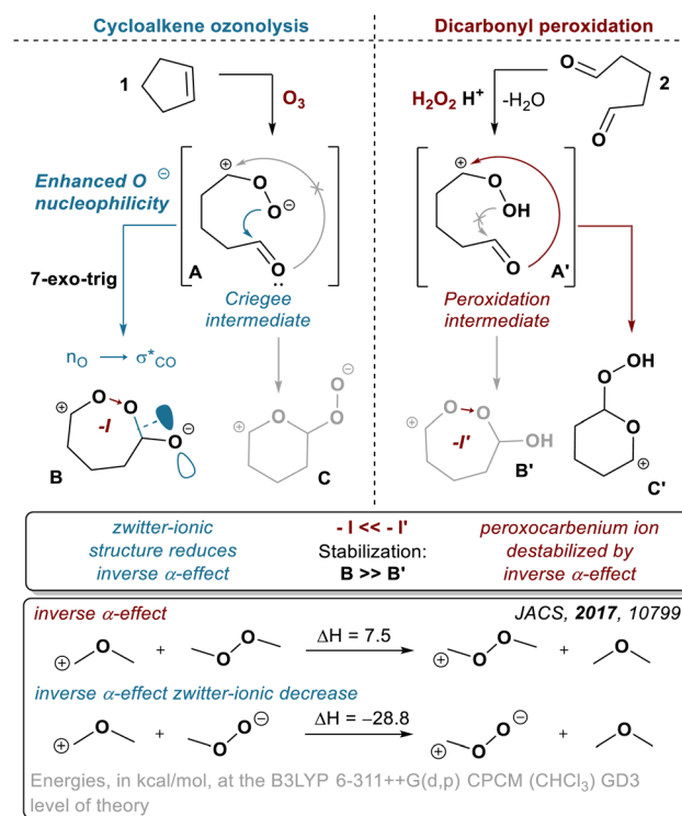
Scheme 11 Comparison of preferred cyclization routes for Criegee intermediate A and peroxy-carbenium intermediate A' .
