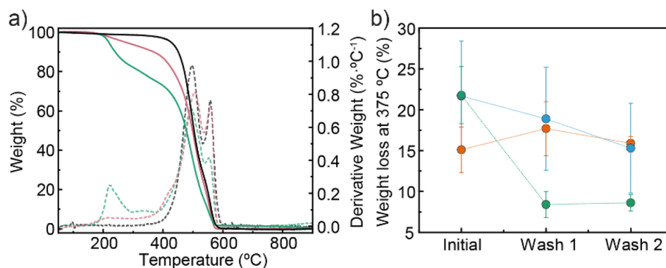
Fig. 4 (a) TGA analysis (air, 10\text{ }^{\circ}\text{C min}^{-1} ) of (6,5)-SWNT (black), eW-SWNT (green) and the supramolecular mixture of (6,5)-SWNTs with eW (pink). (b) TGA weight losses at 375\text{ }^{\circ}\text{C} (air, 10\text{ }^{\circ}\text{C min}^{-1} ) before and after two hot washes in eW-SWNT (green), eW-SWNT submitted to \text{NaBH}_4 treatment (orange) and eR-SWNT (blue).
