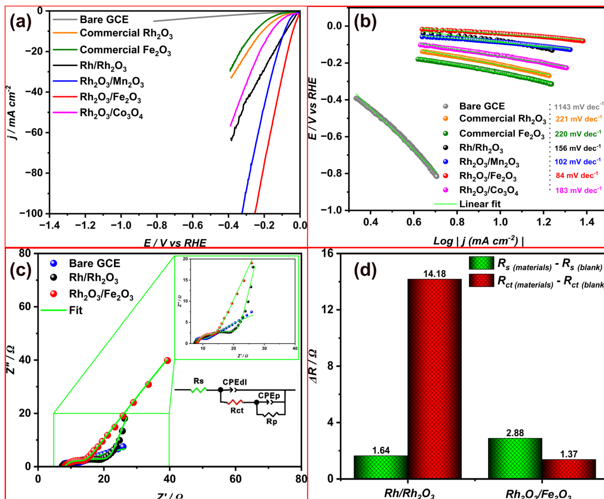
Fig. 5 (a) LSV curves recorded at a scan rate of 100 mV s -1 for commercial Rh _2\text{O}_3 , commercial \alpha\text{-Fe}_2\text{O}_3 , and synthesized Rh/Rh _2\text{O}_3 , Rh _2\text{O}_3/\text{Mn}_2\text{O}_3 , Rh _2\text{O}_3/\text{Fe}_2\text{O}_3 , and Rh _2\text{O}_3/\text{Co}_3\text{O}_4 in 0.5 M \text{H}_2\text{SO}_4 (without iR compensation); (b) corresponding Tafel plots derived from the LSV data; (c) Nyquist plots for Rh/Rh _2\text{O}_3 , Rh _2\text{O}_3/\text{Fe}_2\text{O}_3 , and bare GCE, with insets showing magnified semicircle regions and the equivalent circuit used for fitting; (d) comparative plot of charge transfer resistance ( \Delta R_{\text{ct}} ) values extracted from EIS data for Rh/Rh _2\text{O}_3 and Rh _2\text{O}_3/\text{Fe}_2\text{O}_3 relative to bare GCE.
