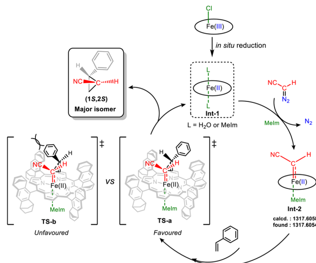
Scheme 8 Plausible mechanism of (+)\text{-D}_4\text{-(por)FeCl} -catalyzed asymmetric cyclopropanation.
