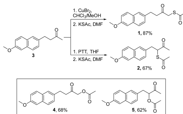
Scheme 1 Synthesis of mercapto-nabumetone derivatives 1 and 2 ; inset: structures of negative controls 4 and 5 (Schemes S1, see the ESI † ).
