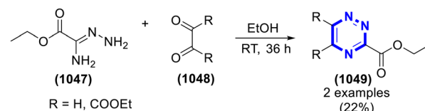
Scheme 291 Synthesis of 1,2,4-triazine-3-carboxylate.
