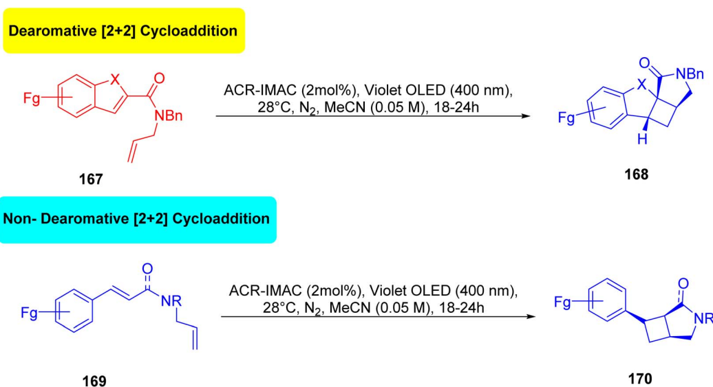
Fig. 69 Non-dearomatizing and dearomatizing intramolecular [2 + 2] photocycloaddition reactions. 254
