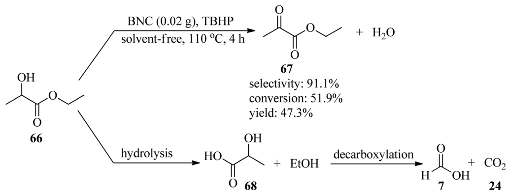
Scheme 21 Preparation of ethyl pyruvate (EP) from ethyl lactate (EL).
