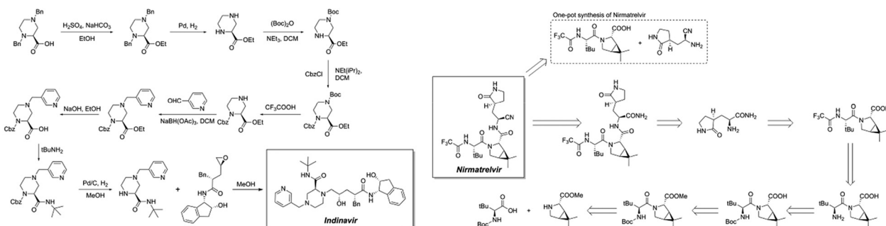
Fig. 4 Retrosynthetic planning of selected small molecular drugs using ASKCOS.
