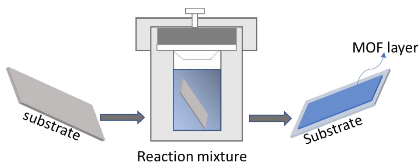
Figure 8. MOF-based electrode construction by direct solvothermal growth.
