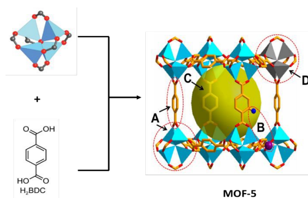
Figure 1. Metal-organic framework catalyst structure where: A is the connecting site for metal clusters and linkers in pristine MOFs, B is a site for grafting metal/non-metals in MOFs by modification, C is a site for encapsulated species in MOF composites and D is sites generated in MOF derivatives upon thermal/chemical conversion. 28 Copyright 2019, Elsevier.
