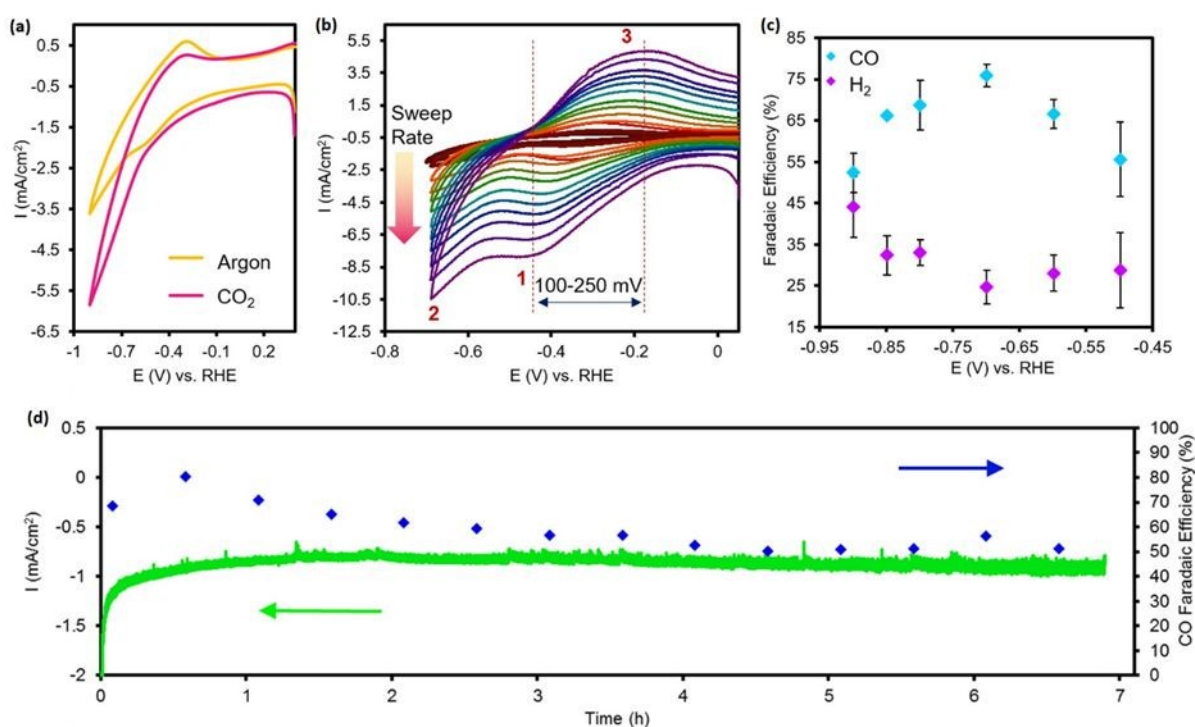
Figure 13. (a) CV scan of the \text{Al}_2(\text{OH})_2\text{TCPP-Co} MOF catalyst showing a current increase in a \text{CO}_2 environment relative to an argon-saturated environment. (b) Varying scan rate with corresponding redox potentials (c) Plot of the faradaic efficiency at the potential range of -0.5 – 0.9 V vs. RHE; (d) MOF stability test with corresponding FE measurement. Reproduced from Kornienko et al. 103 . Copyright 2015, American Chemical Society
