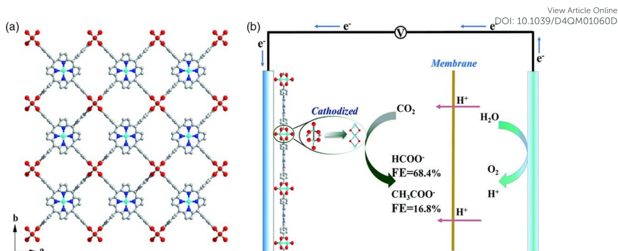
Figure 14. (a) Crystal structure of \text{Cu}_2(\text{CuTCPP}) MOF nanosheets; b) schematic of electrochemical system showing electrocatalytic reduction of \text{CO}_2 on \text{Cu}_2(\text{CuTCPP}) nanosheets. Reproduced with permission from Wu et al. 100 . Copyright 2019, Royal Society of Chemistry.
