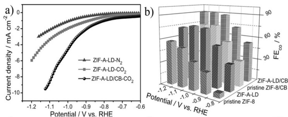
Figure 16. (a) LSV curves of ZIF-8 activated and 1,10-phenanthroline ligand doped product (ZIF-A-LD) in N 2 - and CO 2 -saturated 0.1 M KHCO 3 solution in comparison with ZIF-A-LD/CB b) FE CO . Reproduced from Dou et al. 156 Copyright 2019, Wiley.
