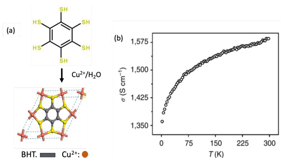
Figure 3. (a) electrically conductive Cu-BHT 2D MOFs designed by \pi -conjugation (b) Electrical conductivity measurement of Cu-BHT film as a function of temperature ranging from 2 to 300 K. Reproduced with permission from Zhu et al. 36 Copyright Springer Nature, 2015.
