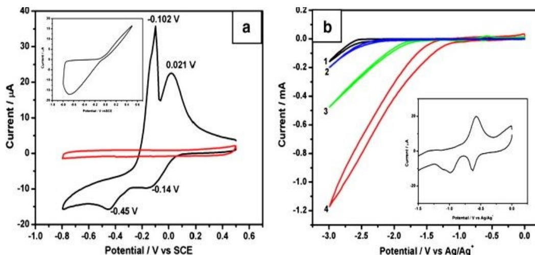
Figure 12. (a) CV readings of Cu 3 (BTC) + GCE (b) CV scan showing redox activities of 1) GCE, 2) GCE in presence of CO 2 , 3) Cu 3 (BTC) 2 + GCE and 4) Cu 3 (BTC) 2 + GCE in CO 2 -saturated 0.01 M TBATFB/DMF. Reproduced from Kumar et al. 112 Copyright 2012, Elsevier
