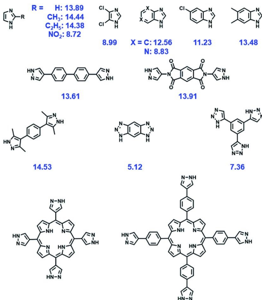
Figure 6. Some representative N donor ligands, with their pK_a s. Reproduced with permission from Ding et al. 63 Copyright Royal Society of Chemistry, 2019
