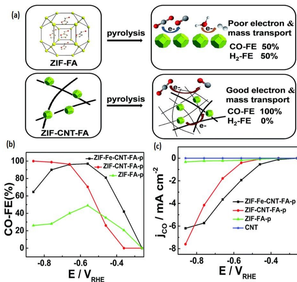
Figure 19. (a) Schematic showing the pyrolysis of ZIFs on multi-walled carbon nanotubes (MWCNT) which aid interparticle conductivity and enhance the mass transport in CO 2 RR. (b)
