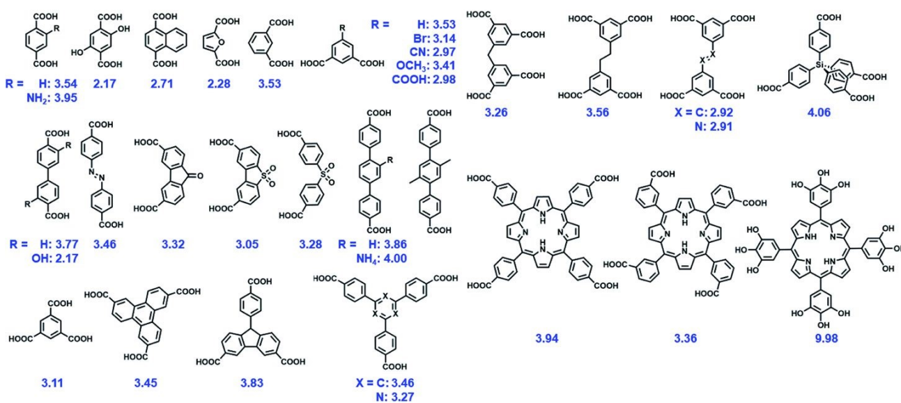
Figure 5. Some representative O donor ligands, with their pK_a s. Reproduced with permission from Ding et al. 63 Copyright Royal Society of Chemistry, 2019
