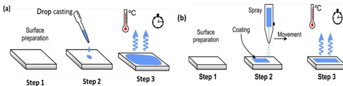
Figure 7. MOF-based electrode construction by (a) drop casting (b) spray coating methods.
