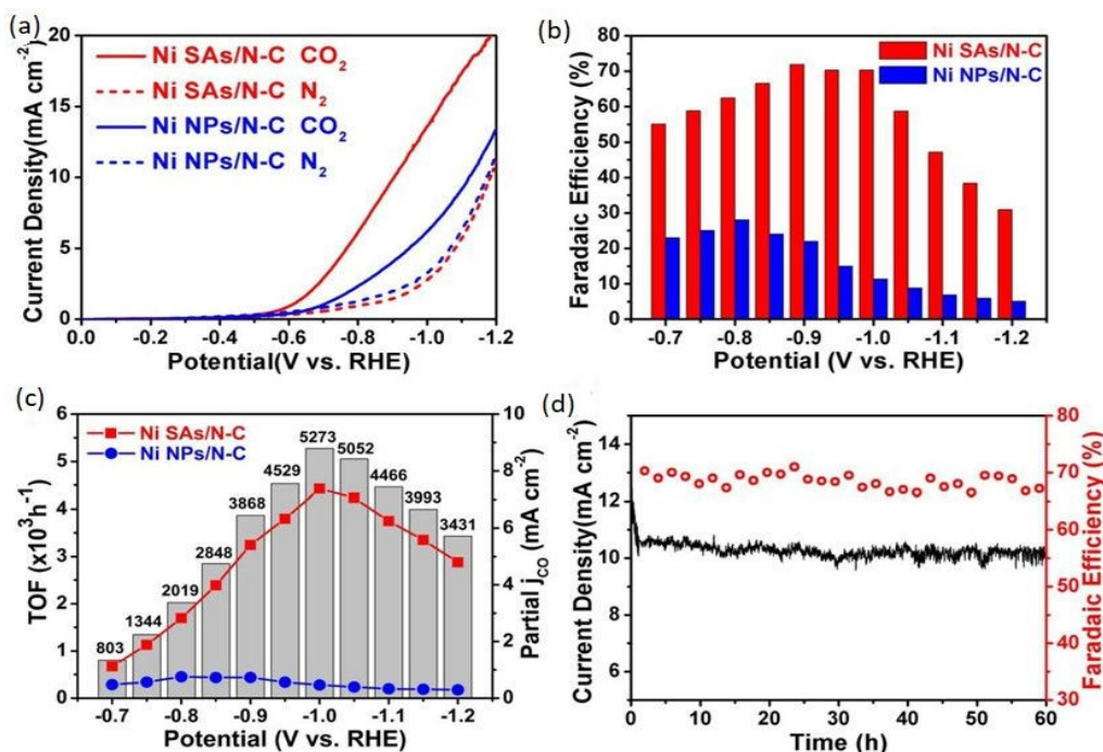
Figure 20. (a) LSV curves in the \text{N}_2 -saturated (dotted line) or \text{CO}_2 -saturated (solid line) 0.5 \text{ M KHCO}_3 electrolyte at a scan rate of 10 \text{ mV s}^{-1} . (b) FEs of CO and (c) partial CO current density plots and TOFs of Ni SAs/N-C and Ni NPs/N-C at different applied potentials. (d) Stability of Ni SAs/N-C at a potential of -1.0 \text{ V vs RHE} for Ni SAs/N-C during 60 h. Reproduced from Zhao et al. 158 . Copyright 2017, American Chemistry Society.
