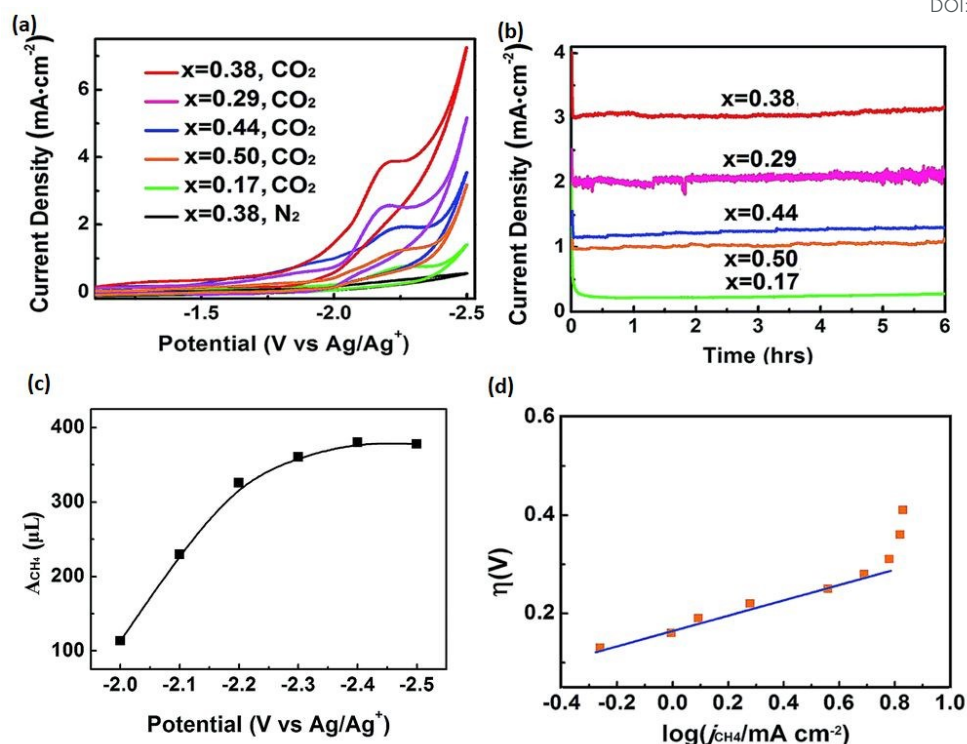
Figure 15. (a) CV scans in CO 2 -saturated and (b) stability test of different Zn-MOF/CP cathodes. (c) Amount of CH 4 ( A_{CH_4} , volume at standard temperature and pressure) generated in 2 h under different potentials. (d) Tafel plot for CH 4 of the Zn-MOF/CP cathode using Zn-MOF synthesized at x = 0.38 . Reproduced from Kang et al. 162 Copyright 2017, Wiley
