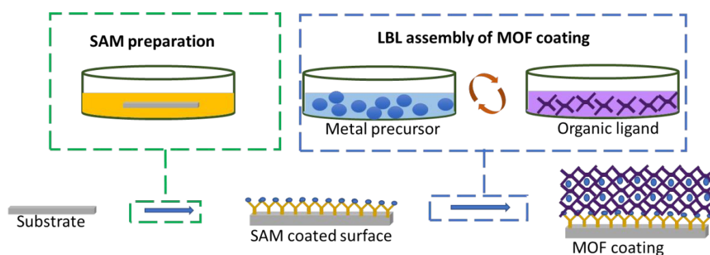
Figure 9. MOF-based electrode construction by liquid phase epitaxy (LPE).
