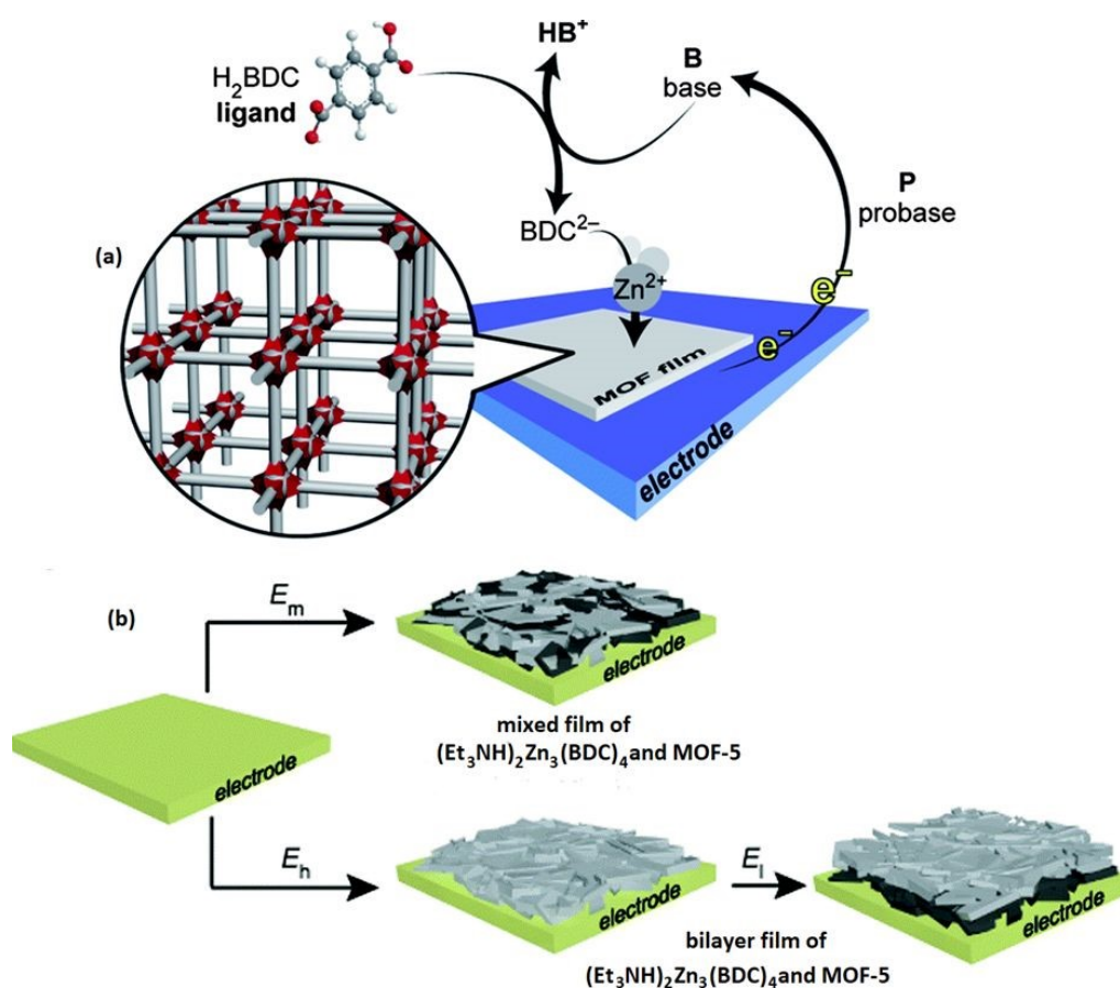
Figure 11. (a) General scheme for the cathodically induced electrochemical deposition of MOFs, involving the reduction of probase (P), the generation of base equivalents (B), the deprotonation of
