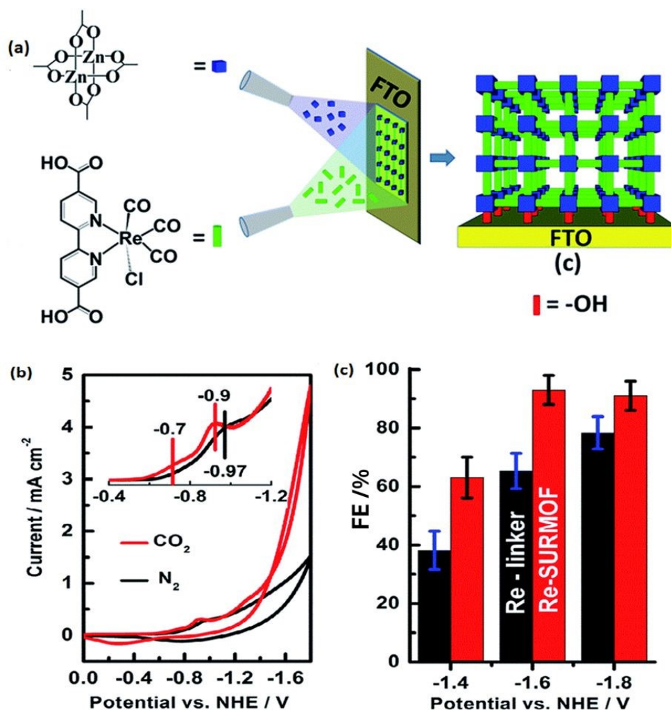
Figure 18. (a) Schematic description of the preparation of a Re-SURMOF on fluorine-doped titanium oxide (FTO) electrode (b) CV scan and (c) FE of the Re-SURMOF and Re-linker at different applied potentials. Reproduced from Ye et al. 124 Copyright 2016, Royal Society of Chemistry.
