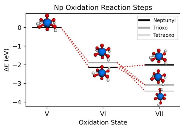
Fig. 8 Diagram describing the formation of a stable \text{Np(VII)} species from \text{Np(V)} oxidation under basic conditions that was originally proposed by Kravchuk et al. 74 The \cdot\text{OH} was determined to be the most likely oxidant and two metastable \text{Np(VI)} complexes were identified before oxidation to the \text{Np(VII)} occurs. Np, O, and H are depicted as blue, red, and white spheres, respectively.
