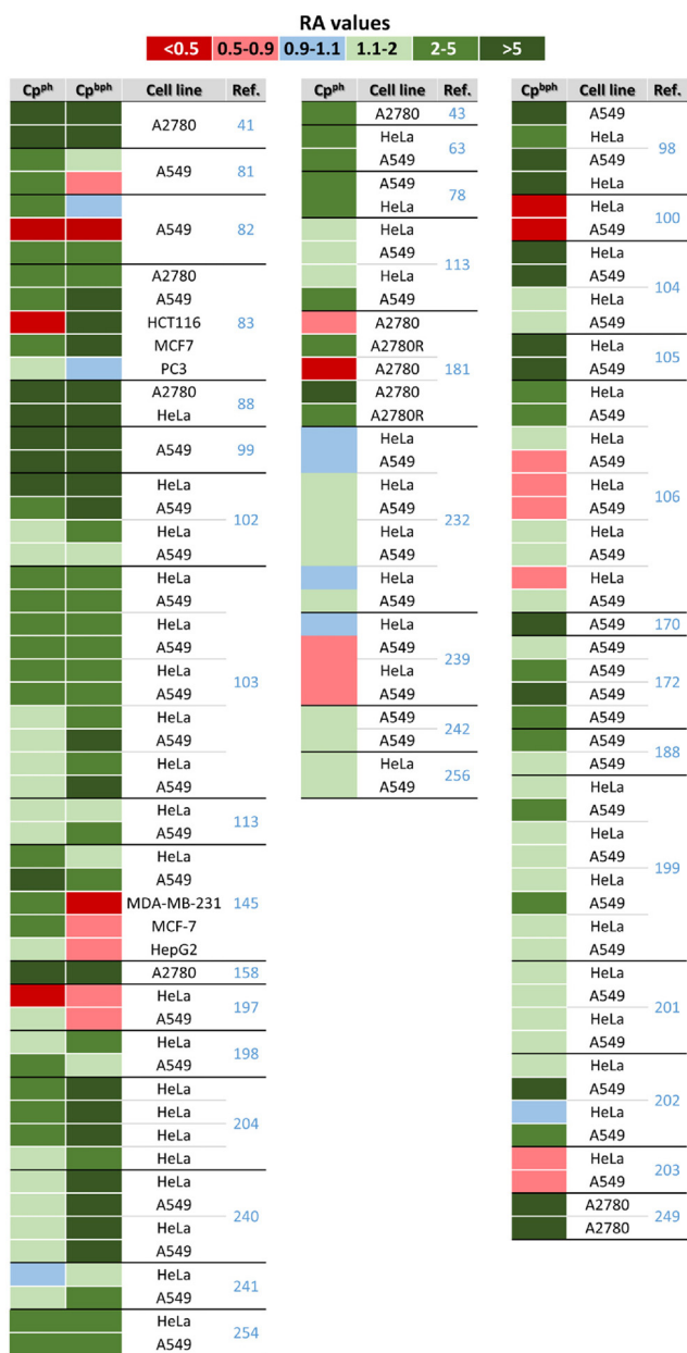
Fig. 32 A comparison of the relative activity (RA) of Cp ph and Cp bph complexes versus their Cp * analogue. RA = IC 50 (Cp * complex)/IC 50 (Cp x complex); Cp * = Cp ph and Cp bph .
