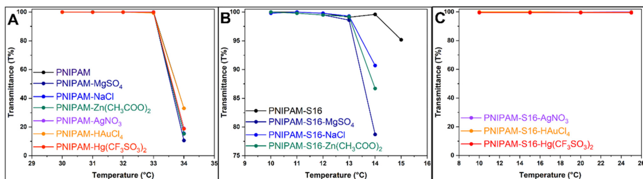
Fig. 5 Transmittance of aqueous solutions of (A) PNIPAM (1.0 mg mL -1 , λ = 700 nm) containing NaCl, Zn(CH 3 COO) 2 , MgSO 4 , Hg(CF 3 SO 3 ) 2 , AgNO 3 and HAuCl 4 . Transmittance of aqueous solutions of PNIPAM-S16 (1.0 mg mL -1 , λ = 700 nm) containing (B) NaCl, Zn(CH 3 COO) 2 and MgSO 4 and (C) Hg(CF 3 SO 3 ) 2 , AgNO 3 and HAuCl 4 .
