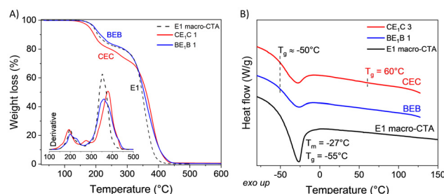
Fig. 7 (A) TGA scans and the relative derivative (inset), and (B) representative DSC second heating scans of E1 macro-CTA and its relative copolymers BEB and CEC.
