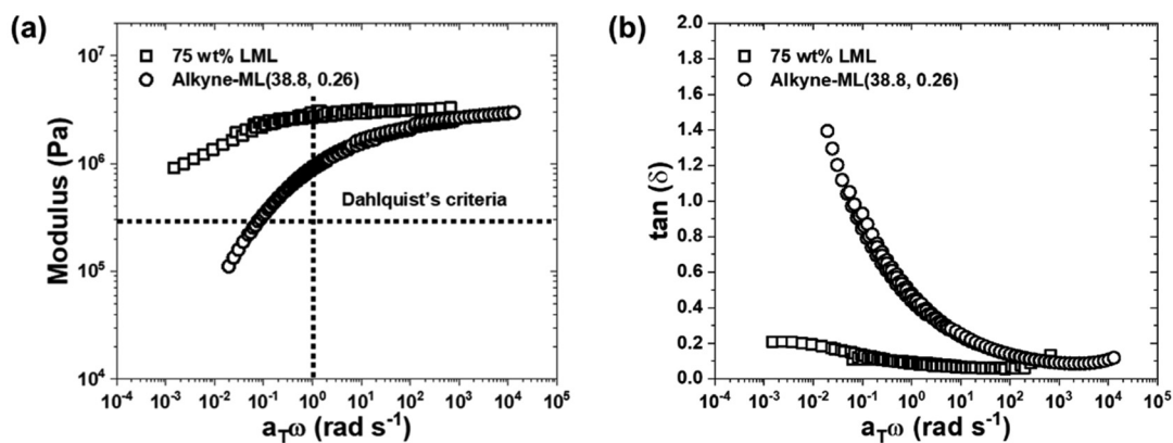
Fig. 5 Master curves for the (a) storage modulus ( G' ) and (b) \tan(\delta) of alkyne-ML(38.8, 0.26) and 75 wt% LML blends after solvent casting. The Dahlquist criterion ( G' = 0.3 MPa at 1 rad s^{-1} ) is marked by dashed lines.
