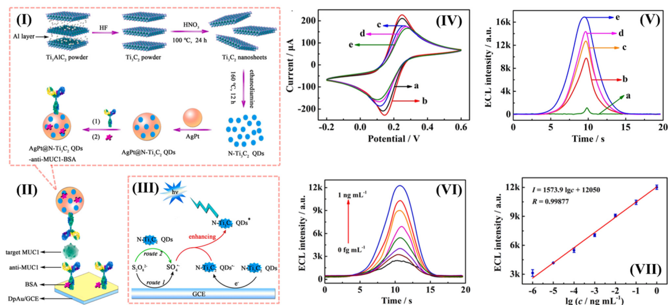
Fig. 11 Schematic representations of a MXene-QD-based ECL sensor probe for MUC1 detection. (I) The synthesis of \text{AgPt}@N\text{-MXene QDs-anti-MUC1-BSA} bioconjugates, where N\text{-MXene QDs} are combined with bimetallic \text{AgPt} nanoparticles and then conjugated with anti-MUC1 antibodies to obtain a highly selective ECL sensor probe. (II) The development of the ECL immunosensor. (III) The possible ECL mechanism of the N\text{-MXene QDs}/\text{S}_2\text{O}_8^{2-} system; here MXene QDs act as luminophores in the presence of the co-reactant potassium persulphate, producing significantly enhanced luminescence via intermediate generation. (IV) The CV response of each modified electrode: a bare GCE (a), DpAu/GCE (b), anti-MUC1/DpAu/GCE (c), BSA/anti-MUC1/DpAu/GCE (d), and MUC1/BSA/anti-MUC1/DpAu/GCE (e), confirming the step-by-step modification of the sensor probe. (V) A comparison of ECL responses after each modification of the sensor showing the ECL intensities of (a) N\text{-Ti}_3\text{C}_2\text{ QDs} in \text{S}_2\text{O}_8^{2-} solution, (b) N\text{-Ti}_3\text{C}_2\text{ QDs} in \text{S}_2\text{O}_8^{2-} solution with Ag nanoparticles, (c) N\text{-Ti}_3\text{C}_2\text{ QDs} in \text{S}_2\text{O}_8^{2-} solution with Pt nanoparticles, and (d) N\text{-Ti}_3\text{C}_2\text{ QDs} in \text{S}_2\text{O}_8^{2-} solution with AgPt nanoparticles, which demonstrates the highest ECL response due to the synergistic effect of bi-metallic AgPt nanoparticles. (VI) The ECL responses of the fabricated immunosensor to various concentrations of MUC1, highlighting the concentration-dependent increase in the ECL signal due to antigen-antibody interactions. (VII) The calibration plot of the developed sensor for MUC1 detection, representing the sensitivity and stability of the sensor probe. Reproduced with permission from ref. 242; copyright 2022, ELSEVIER.
