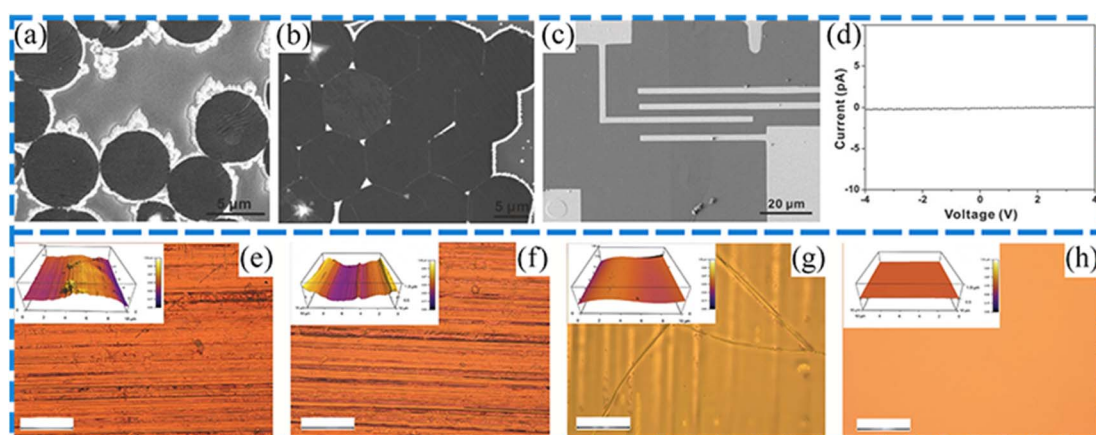
Fig. 12 (a) SEM image of multiple circular h-BN domains; 117 (b) SEM image shows the h-BN SASCA with circular h-BN domains on the edges; 117 (c) SEM image of the h-BN electronic device configuration; 117 (d) the current–voltage curve of h-BN showing excellent electrical insulation properties; 117 (e–h) optical microscope images and Raman spectra of different copper substrates, (e) as-received, (f) 10% HNO 3 acid etched, (g) annealed at 1000 °C, and (h) melted at 1100 °C, the scale bar is 50 μm. The inset in each of the images shows the 3D AFM height profile across a 10 × 10 μm 2 area. The color bar is within the 0 to 1 μm range in all the insets. 116
