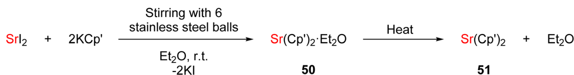
Fig. 23 The synthesis of unsolvated \text{Sr(Cp')}_2 . 126
