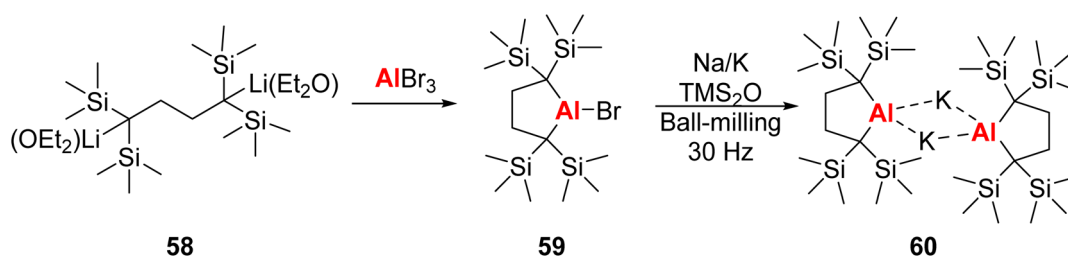
Fig. 26 Synthesis of non-solvated dialkylaluminum anion, [K(AlR_2)_2]_2 via mechanochemical method. 131
