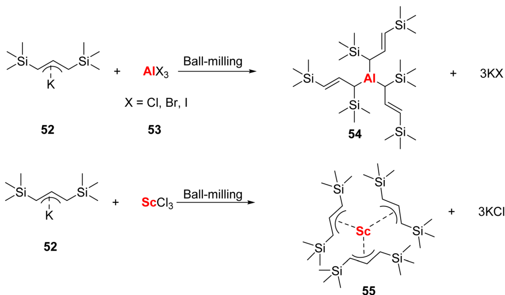
Fig. 24 Synthesis of unsolvated [1,3-(\text{SiMe}_3)_2\text{C}_3\text{H}_3]_3(\text{Al, Sc}) . 129
