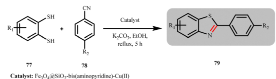
Catalyst: \text{Fe}_3\text{O}_4@SiO_2 -bis(aminopyridine)- \text{Cu}(II)
