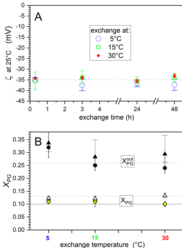
Fig. 2 Properties of aLUVs of \text{SOPC}^{\text{in}}|+20 \text{ mol\% DPPG}^{\text{out}} prepared by exchange between SOPC “acceptor” vesicles with nearly DPPG-saturated m \beta CD solution as a function of exchange time (A) and exchange temperature (B). Panel A shows data of batch 5 (see Table S8† for detailed data) as a function of exchange temperature (see plot) and exchange time (abscissa). The zeta potential, \zeta , is related to the DPPG-based charge density in the outer leaflet; it is always measured at 25 °C to eliminate effects of varying membrane area. Panel B displays total DPPG mole fractions, X_{\text{PG}} , obtained using Fig. S3† from \zeta of scrambled aLUVs (open triangles, batch 4) and HPLC (yellow hexagons, batches 1–3). PG mole fractions in the outer leaflet of aLUVs, X_{\text{PG}}^{\text{out}} , are obtained from \zeta for batch 4 (solid black triangles) and batches 1–3 (solid black hexagons). Errors of HPLC-based data are s.d. of triplicate measurements. Errors of \zeta -based data reflect lower and upper limits of the 95% confidence interval of the calibration curve, Fig. S3.†
