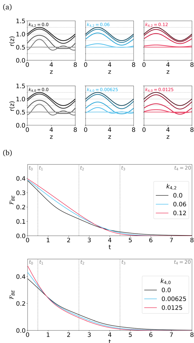
Fig. 1 (a) Time evolution of axisymmetric simulations for different parameters for k_{4,2} and k_{4,0} starting from the same periodic solution r_0(z) = \frac{1}{4}\sin(\frac{\pi}{4}z) + 1 at t_0 . The evolution goes from dark to light converging to a tube with r(z) = 0.5 . The depicted time instances are marked in (b). (b) Corresponding time evolution of the bending energy for different values of k_{4,2} and k_{4,0} . Parameters are k_{2,0} = 0.05 and \mathcal{H}_0 = -2 .
