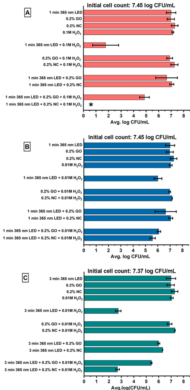
Fig. 5 The E. coli inactivation efficacy values of the combined treatments (365 nm + NP + H_2O_2 ): (A) 0.1 M H_2O_2 and 1 min LED treatment, (B) 0.01 M H_2O_2 and 1 min LED treatment and (C) 0.01 M H_2O_2 and 3 min LED treatment. Results are shown as mean \pm standard deviation of triplicate independent experiments. Here, N_0 represents the CFU mL -1 in control and N represents the CFU mL -1 in the treated samples. Error bars indicate the standard deviation ( n = 3 ). An asterisk (*) indicates the reduction of cell counts below the detection limit.
