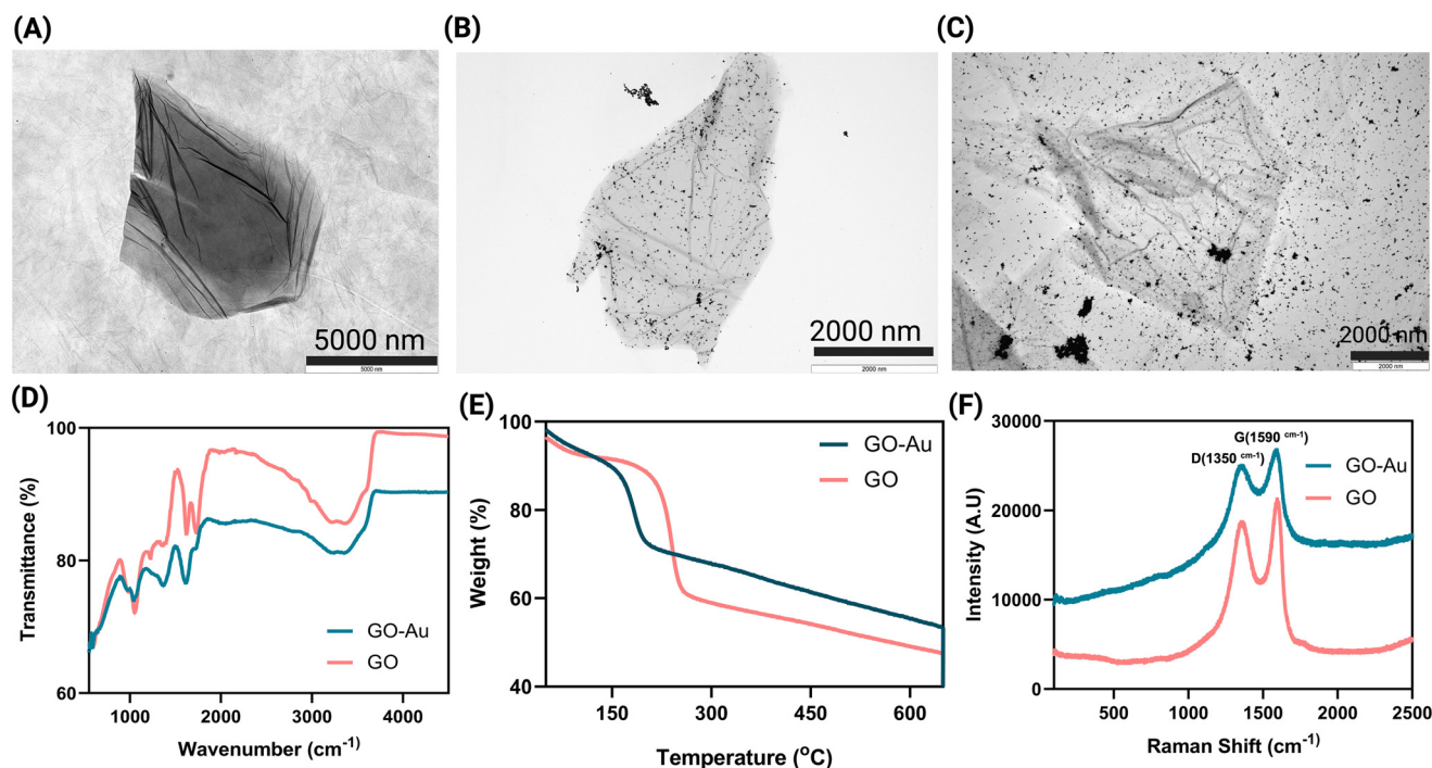
Fig. 1 Physicochemical characterization and stability of GO and GO-Au nanohybrids. (A) Transmission electron microscopy (TEM) image of GO showing its layered structure with a wrinkled morphology. (B) and (C) TEM images of the GO-Au nanohybrid, demonstrating the uniform distribution of AuNPs on the GO sheets. (D) Fourier-transform infrared (FTIR) spectra of GO and GO-Au nanohybrids. For GO, characteristic peaks include the C=O stretching at \sim 1730\text{ cm}^{-1} and C-O stretching at \sim 1220\text{ cm}^{-1} . For GO-Au, the C=O peak is less intense, indicating interaction between AuNPs and oxygen-containing groups on GO. (E) TGA curves showing weight loss profiles of GO and GO-Au. GO exhibits a weight loss at around 200\text{--}300\text{ }^{\circ}\text{C} due to decomposition of oxygen-containing functional groups, while GO-Au displays a more gradual weight loss, indicating enhanced thermal stability. (F) Raman spectra of GO and GO-Au nanohybrids, highlighting the D ( \sim 1350\text{ cm}^{-1} ) and G ( \sim 1590\text{ cm}^{-1} ) bands. The D/G intensity ratio is higher for GO-Au, indicating structural changes due to AuNP decoration.
