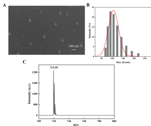
Fig. 1 Characterization of C_{60} . (A) SEM image, (B) DLS image, (C) time-of-flight mass spectrum.
