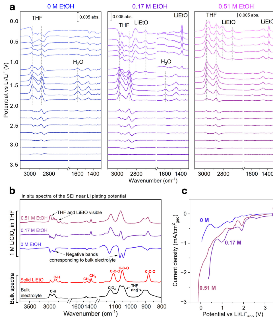
Fig. 2 (a) FTIR spectra of the working electrode during the initial SEI-forming cathodic potential scan from OCP towards the apparent Li plating potential in an electrolyte consisting of 1 M LiClO 4 in THF with 0 M, 0.17 M and 0.51 M ethanol (0%, 1% and 3% by volume), and <2.5 mM (~45 ppm) water. The working electrode consists of a 50 nm sputtered Cu film on top of an Au adhesion layer deposited on a 22 mm diameter hemispherical ZnSe prism. Spectra are all relative to a background spectrum taken at the initial OCP. (b) Comparison of the spectra measured closest to 0 V Li/Li + in each case with measured ATR spectra of the bulk electrolyte and solid LiEtO for reference. (c) LSVs measured in electrolytes of 0 M, 0.17 M and 0.51 M ethanol at a scan rate of -5 \text{ mV s}^{-1} . Working electrode potentials are corrected for Ohmic drop ( R_U = 120 \Omega ). The IR cell is a single compartment with a 1 cm 2 Pt mesh counter and Pt wire reference, each with approximately 1 cm separation (Fig. S1, ESI†).
