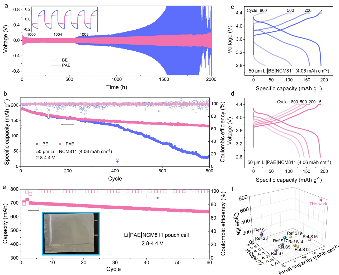
Fig. 6 Practical electrochemical performances. (a) Cycling performance of symmetric LMBs with various electrolytes at a current density of 0.5 \text{ mA h cm}^{-2} ( 0.5 \text{ mA h cm}^{-2} ). The inset provides a detailed view of the 1000th to the 1010th cycle. (b) Cycling performance of 50 \mu\text{m Li} \parallel \text{NCM811} ( 4.06 \text{ mA h cm}^{-2} ) cells with various electrolytes cycled at 0.2\text{C} charge and 0.3\text{C} discharge ( 1\text{C} = 200 \text{ mA g}^{-1} ). (c) Charge-discharge voltage profiles of the 50 \mu\text{m Li} \parallel \text{NCM811} ( 4.06 \text{ mA h cm}^{-2} ) cell using BE. (d) Charge-discharge voltage profiles of the 50 \mu\text{m Li} \parallel \text{NCM811} ( 4.06 \text{ mA h cm}^{-2} ) cell using PAE. (e) Cycling performance of the \text{Li} \parallel \text{NCM811} ( 692 \text{ mA h} ) pouch cell with an energy density of 397 \text{ W h kg}^{-1} (inset: the digital photo of the pouch cell; 0.2\text{C} charge/ 0.3\text{C} discharge). (f) Performance comparison of the cell with PAE against published studies involving SPEs (more data are detailed in Table S5, ESI†).
