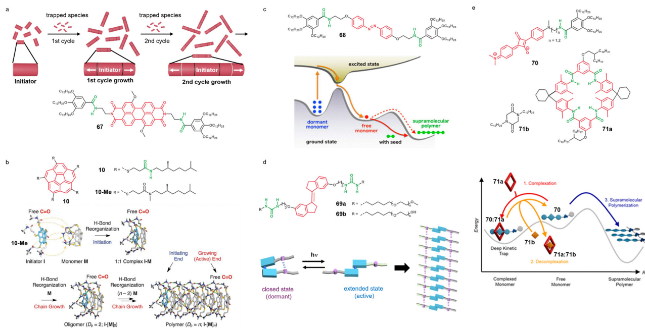
Fig. 18 (a) Schematic representation of the living supramolecular polymerization process and the molecular structure of PBI 67 . The initiator refers to a seed or a single molecule. The trapped species can consist of kinetically trapped monomeric aggregated species. (b) Molecular structures of compounds 10 and 10-Me , and a schematic representation of the supramolecular polymerization process triggered by adding small amounts of 10-Me into a solution of 10 (reproduced from ref. 137 with permission of the American Association for the Advancement of Science, copyright 2015). (c) Molecular structure of compound 68 and the corresponding self-assembly energy landscape of the light controlled self-assembly process (reproduced from ref. 314 with permission of the American Chemical Society, copyright 2016). (d) Molecular structure of compounds 69a,b and the schematic illustration of the light controlled self-assembly process (reproduced from ref. 315 with permission of the American Chemical Society, copyright 2021). (e) Molecular structures of compounds 70 , 71a and 71b , and the corresponding self-assembly energy landscape for the controlled supramolecular polymerization process (reproduced from ref. 317 with permission of the American Chemical Society, copyright 2023).
