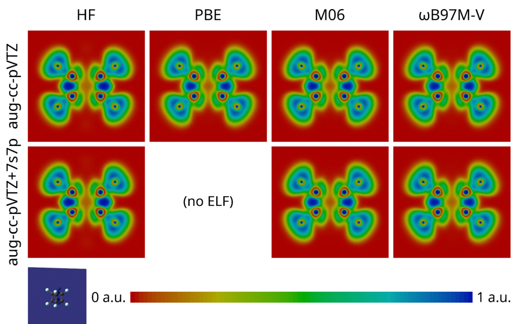
Fig. 4 Isocontour plots of the anionic ELF at the equilibrium geometry of the C_8F_8 anion, for different methods and basis sets (specified in the figure). The ELFs were plotted in a plane through the center of the molecule and containing two opposite C–C bonds and four C–F bonds (see the inset at bottom left).
