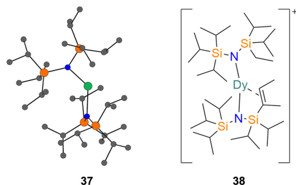
Fig. 5 (left) Solid-state structure of the cation in [\text{Dy}(\text{N}(\text{Si}^i\text{Pr}_3)_2)_2][\text{Al}(\text{OC}(\text{CF}_3)_3)_4] ( 37 ). Dysprosium(III) = turquoise, silicone = orange, nitrogen = blue, and carbon = grey; hydrogen atoms have been omitted for clarity. (right) Structure of the cation in [\text{Dy}(\text{N}(\text{Si}^i\text{Pr}_3)(\text{Si}^i\text{Pr}_2\text{-C}(\text{CH}_3)=\text{CHCH}_3))_2][\text{Al}(\text{OC}(\text{CF}_3)_3)_4] ( 38 ), showcasing the weak \eta^2 -alkene coordination. 49,53
