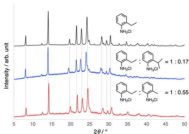
Fig. 5 Formation of mixed crystals with 2-substituted anilinium chlorides. PXRD patterns (CuKα, rt) of 1 (top) and mixed crystals with o -toluidinium chloride (bottom) and 2-isopropylanilinium chloride (middle) with molar ratios shown in the figure, which is estimated through 1 H NMR analysis of the crystals dissolved in DMSO- d 6 .
