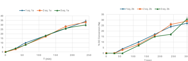
Scheme 2 (a) Competition experiments: 0.50 mmol aryl chloride, 1.00 mmol 2a . (b) Experiments conducted at the 0.50 mmol scale, 60 °C, in 2 mL toluene, with 1.25 mol% [Pd(1-MeNAP)Br] 2 and 2.5 mol% IPent Cl HCl: yield of 3aa vs time using increasing eq. of 1a (left) and conversion of 1a vs. time using increasing eq. of 2b (right). GC yield/conversion using tetradecane as an internal standard. Each datapoint represents the average of two runs.
