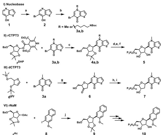
Scheme 1 Synthesis of nucleobases (I), rCTPT3 TP (including CC of 3a and 3b ) (II), dCTPT3 TP (III) and rNaM TP (VI). Conditions for (I): nucleobase 3a , functionalized nucleobase 3b . (a) NBS, AcOH, r.t., 20 h, 99%; (b) for 3a with R = Me: Mel, K 2 CO 3 , DMF, r.t., 20 h, 90%; for 3b (with R = (CH 2 ) 4 NBoc): NBoc-(CH 2 ) 4 -I, K 2 CO 3 , DMF, 50 °C, 24 h, 97%. Conditions for (II): (c) for 4a with R = Me: 4CzIPN (1 mol%), NiBr 2 ·DME (5 mol%), 4,4-diOMe-bipyridine (7 mol%), Na 2 CO 3 , dioxane, 84 °C, h \nu (467 nm), 10 h, 17%; for 4b (with R = (CH 2 ) 4 NBoc): 4CzIPN (1 mol%), NiBr 2 ·DME (5 mol%), bpy (7 mol%), Na 2 CO 3 , dioxane, 84 °C, h \nu (467 nm), 10 h, 11%; (d) p -toluenesulfonic acid, DCM/MeOH, r.t., 20 h; (e) NaOMe, MeOH, r.t., 20 h 95% (2 steps); (f) enzymatically, 90%. Conditions for (III): (g) PdCl 2 (dppf) 3 , Et 3 N, ACN, 100 °C, 72 h; (h) NaHB(OAc) 3 , AcOH/ACN, 0 °C, 2 h, 6% (2 steps); (i) enzymatically ( dRibo enzyme mix, BioNukleo ), 7.5%. Conditions for (VI): (j) TMSBr, Zn, Ni(acac) 2 , THF, 0 °C to r.t. 19 h, 25%.
