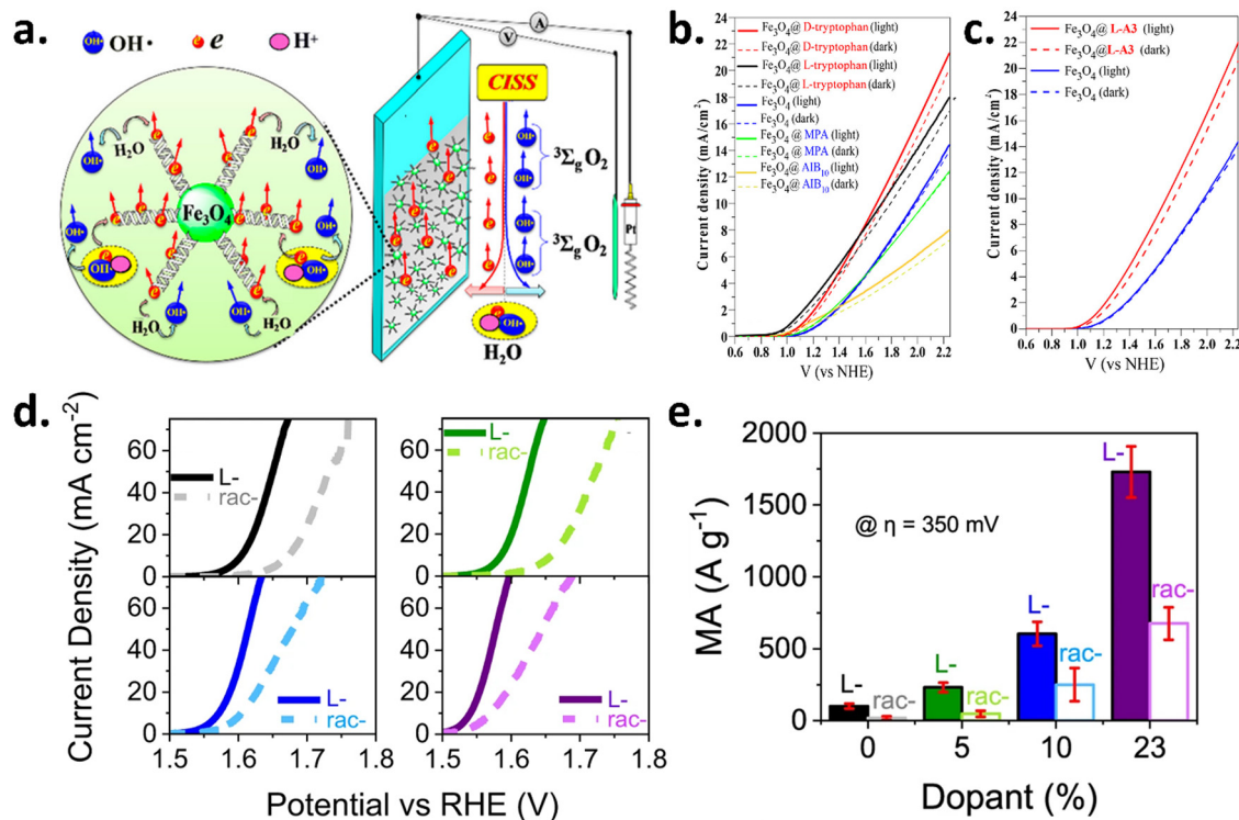
Fig. 6 Chiral functionalization of Fe 3 O 4 and Co 3 O 4 -based nanoparticles and enhancement of spin-selectivity for the OER. (a) Schematic of chiral-functionalized electrodes, where the C 1 S 1 S 2 effect enhances the OER via triplet oxygen production. (b) Photocurrent and dark current densities for Fe 3 O 4 NPs linked to chiral (D- and L-tryptophan) and achiral (mercaptopyronic acid, azo isobutyric acid) molecules, compared to pure Fe 3 O 4 NPs. (c) Photocurrent density of Fe 3 O 4 NPs linked to chiral L-A3 versus pure Fe 3 O 4 NPs. (d) LSV plot showing undoped (black) and iron-doped Rac- (dashed) and L-cobalt oxide (solid) nanoparticle catalysts in Nafion, with doping levels of 5% (green), 10% (blue), and 23% (purple), measured in 1 M NaOH. (e) Mass activity (MA) comparison of Rac- (open symbols) and L-cobalt oxide (filled symbols) nanoparticle catalysts in Nafion. Figures are adopted from ref. 24 and 26 with permission from American Chemical Society © 2018 and Nature © 2023.
