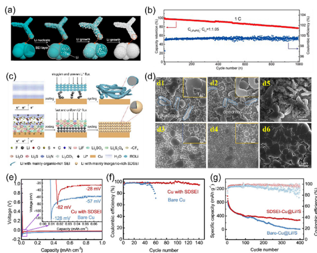
Fig. 3 (a) Illustration of the deposition of Li. (b) Long-term performance of the full cell. 96 (c) Illustrations of the Li deposition behavior on two substrates. (d) SEM images of the 1st Li on a Cu substrate without or with a salt-derived SEI (donated as SDSEI) film at different areal capacities. (e) Comparison of different substrates at 0.5 \text{ mA cm}^{-2} after the 1st Li nucleation. (f) CE at 0.5 \text{ mA cm}^{-2} for Li deposited on a bare Cu substrate and on the Cu substrate with the SDSEI film. (g) Electrochemical performance of different batteries. 97
