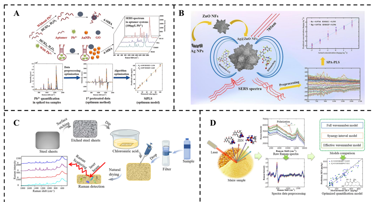
Fig. 9 (A) A rapid and sensitive SERS method for detecting \text{Pb}^{2+} in food established by aptamer regulated gold nanoparticle reduction. 122 (B) Schematic description of deltamethrin residue detection in wheat by Ag@ZnO NF-based surface-enhanced Raman spectroscopy coupled with chemometric models. 123 (C) Schematic illustration of the preparation of Au nanostars and the sample detection process. 124 (D) Flowchart of the main data processing procedures for predicting zearalenone in maize by Raman spectroscopy. 125
