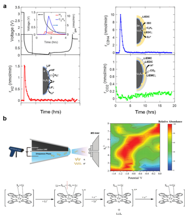
Fig. 13 (a) The DEMS measurements of generated gases in the first formation cycle of a \text{Li} -graphite cell. Insets show the proposed mechanism of \text{LiF} deposition, \text{LiEDC} deposition, and the \text{LiEMC} chemical formation mechanism. Reprinted with permission from ref. 122. Copyright (2022) American Chemical Society. (b) Schematic of the EC-MS setup, relative abundance distribution of various polysulfides at various potentials estimated from the EC-MS data, and the proposed pathway of the electrolytic polysulfide conversion process with CoPc as an electrocatalyst. Reprinted with permission from ref. 124. Copyright (2021) Wiley-VCH.
