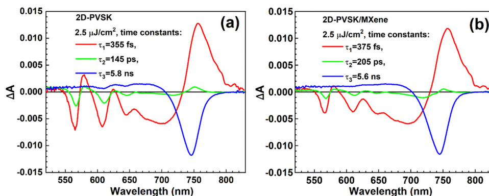
Fig. 7 Wavelength-dependant amplitudes of the indicated time constants from a 3-exponential global fit of TA data excited from HTL side at 475 nm with 2.5 \mu\text{J cm}^{-2} pump fluence for the cells: (a) without MXene and (b) with MXene.
