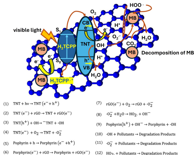
Fig. 31 Diagram depicting the photocatalytic activity of the TCPP/RGO/ \text{TiO}_2 nanotubes = TNT) during the degradation of MB pollutants, including the light-initiated reactions within this photocatalytic system. Adapted with permission from ref. 150. Copyright 2016 Hydrogen Energy Publications LLC.
