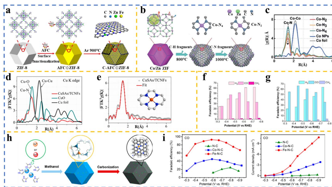
Fig. 8 (a) Schematic of Fe-N doped porous carbon synthesized by adding ammonium ferric citrate (AFC) to as-synthesized ZIF-8, followed by pyrolysis. Reproduced with permission. 194 Copyright 2017, Elsevier. (b) Synthesis process of Co-N 4 and Co-N 2 active sites using Co/Zn ZIF followed by pyrolysis. (c) EXAFS spectra demonstrating the atomic dispersion of Co atoms in Co-N 2 , Co-N 3 , and Co-N 4 , confirming the lowest N coordination number in Co-N 2 . Reproduced with permission. 50 Copyright 2018, Wiley-VCH. (d) Fourier transform (FT) at R space showing Cu-N. (e) EXAFS data fitted of CuSAs/TCNFs. Reproduced with permission. 173 Copyright 2019, the American Chemical Society. Electrochemical performance comparison: faradaic efficiency at different applied potentials for (f) MnSA/NC and (g) MnSA/SNC. Reproduced with permission. 195 Copyright 2021, the American Chemical Society. (h) Schematic of the formation of Fe-N-C and Co-N-C using Fe- and Co-doped ZIF-8. (i) Comparative analysis of CO faradaic efficiency and partial current densities across N-doped carbon, Co-N-doped carbon, and Fe-N-doped carbon. Reproduced with permission. 162 Copyright 2018, the American Chemical Society.
