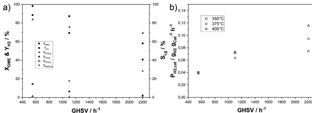
Fig. 7 Effect of GHSV on (a) DME conversions, hydrogen yield and C 1 selectivities at 350 °C; (b) catalyst mass related hydrogen productivities at 350–400 °C ( p = 2 bar(a); molar ratio of n_{H_2O} : n_{DME} : n_{N_2} = 5 : 1 : 1.5 ; m_{In_2O_3/ZrO_2} = 36 g (3 wt% indium content); m_{\gamma-Al_2O_3} = 9 g).
