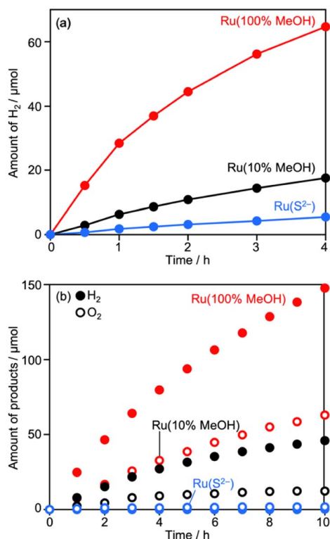
Fig. 3 Photocatalytic (a) \text{H}_2 evolution and (b) Z-WS using \text{Cr}_2\text{O}_3 (1.2 wt%)/Ru (0.5 wt%)/CLTO prepared under different photodeposition conditions. Photocatalyst: 0.2 g for (a) and 0.05 g each for (b); reactant solution: 10 vol% methanol for (a) and 0.1 mM \text{Co}(\text{bpy})_3\text{SO}_4 for (b), 160 mL; light source: 300 W Xe lamp ( \lambda > 420 \text{ nm} ).
